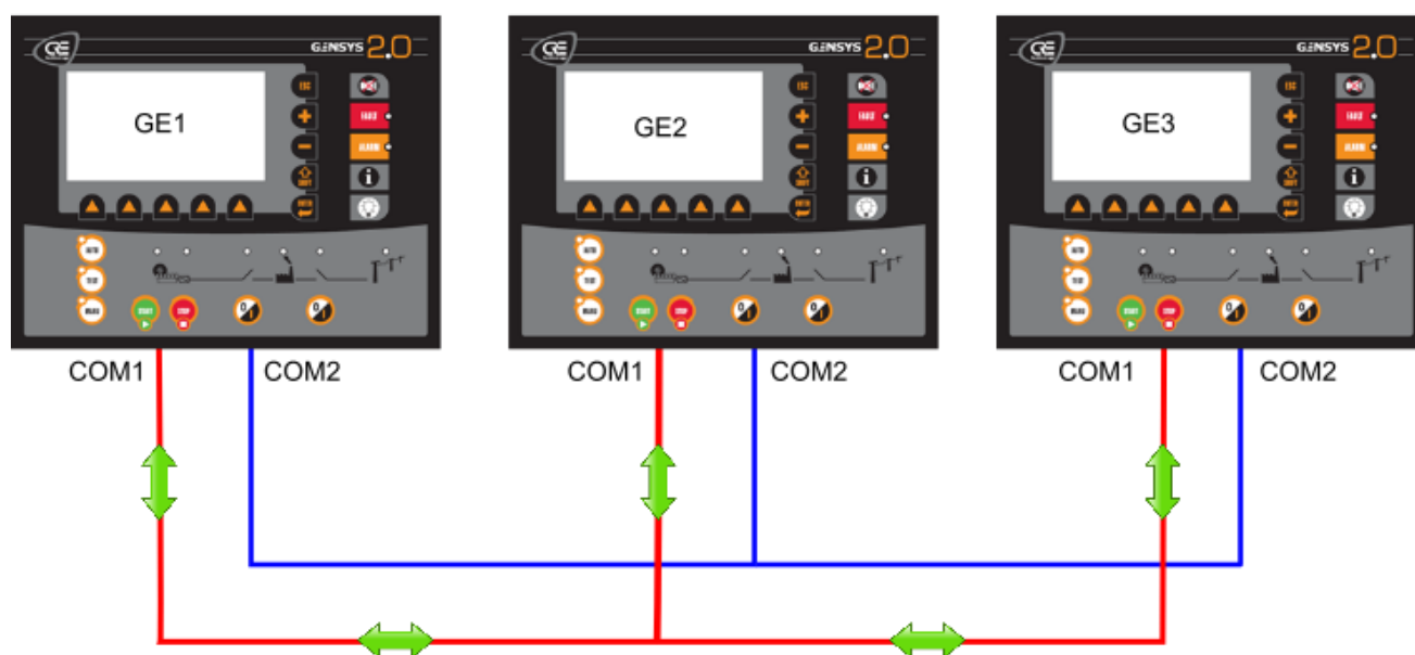
FIGURE 79 - REDONDANCE DE BUS CAN INTER-GENSYS COM1-> COM2 (1/2)
