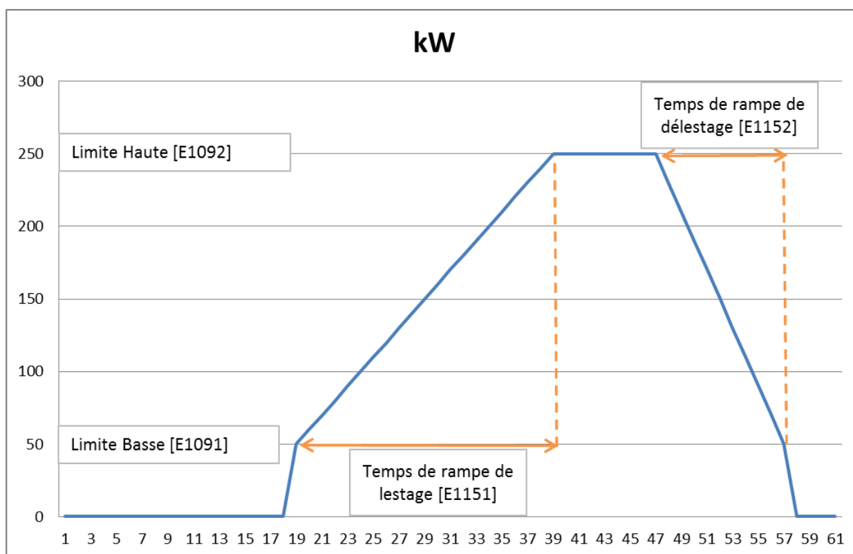
FIGURE 95 - CALCUL RAMPE DE LESTAGE/DÉLESTAGE
