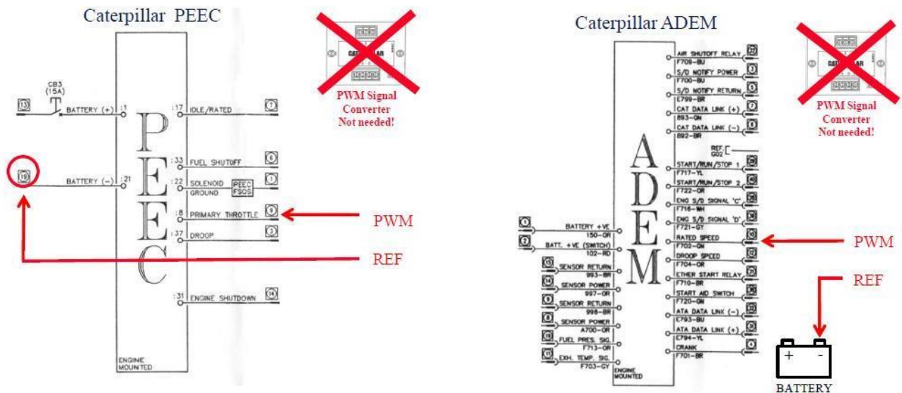
FIGURE 42 - CONNEXION CATERPILLAR PEEC ET ADEM
