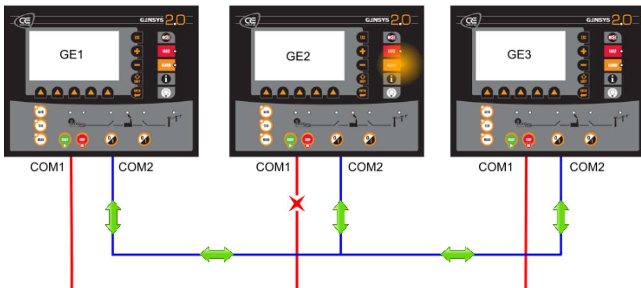
FIGURE 80 - REDONDANCE DE BUS CAN INTER-GENSYS COM1-> COM2 (2/2)
