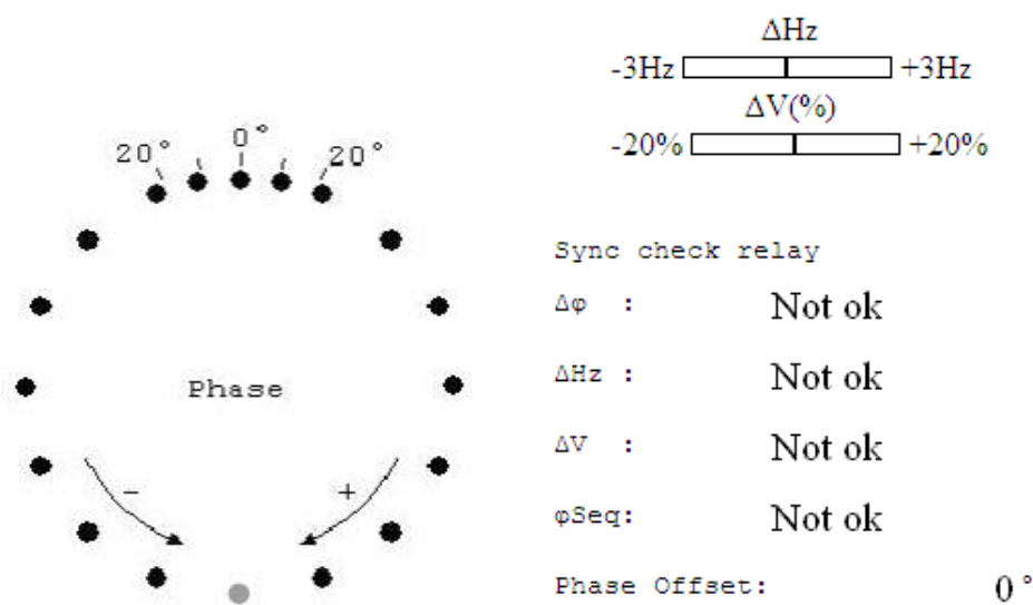
FIGURE 94 - SYNCHRONOSCOPE
