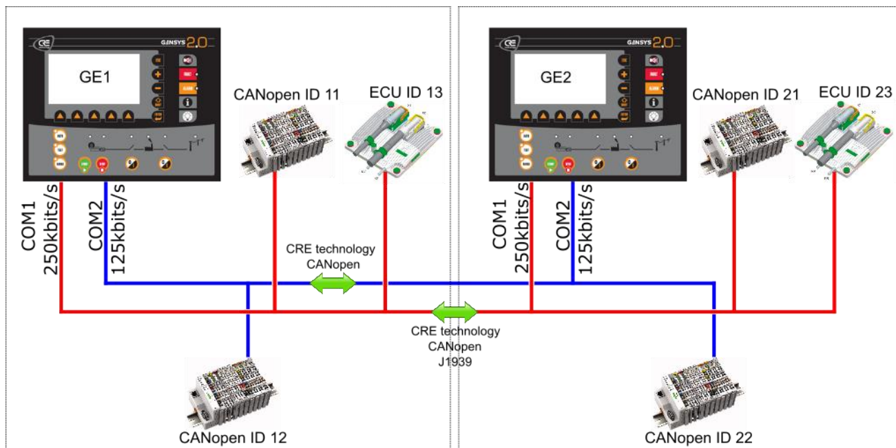
FIGURE 83 - EXEMPLE DE REDONDANCE MULTIPLE
