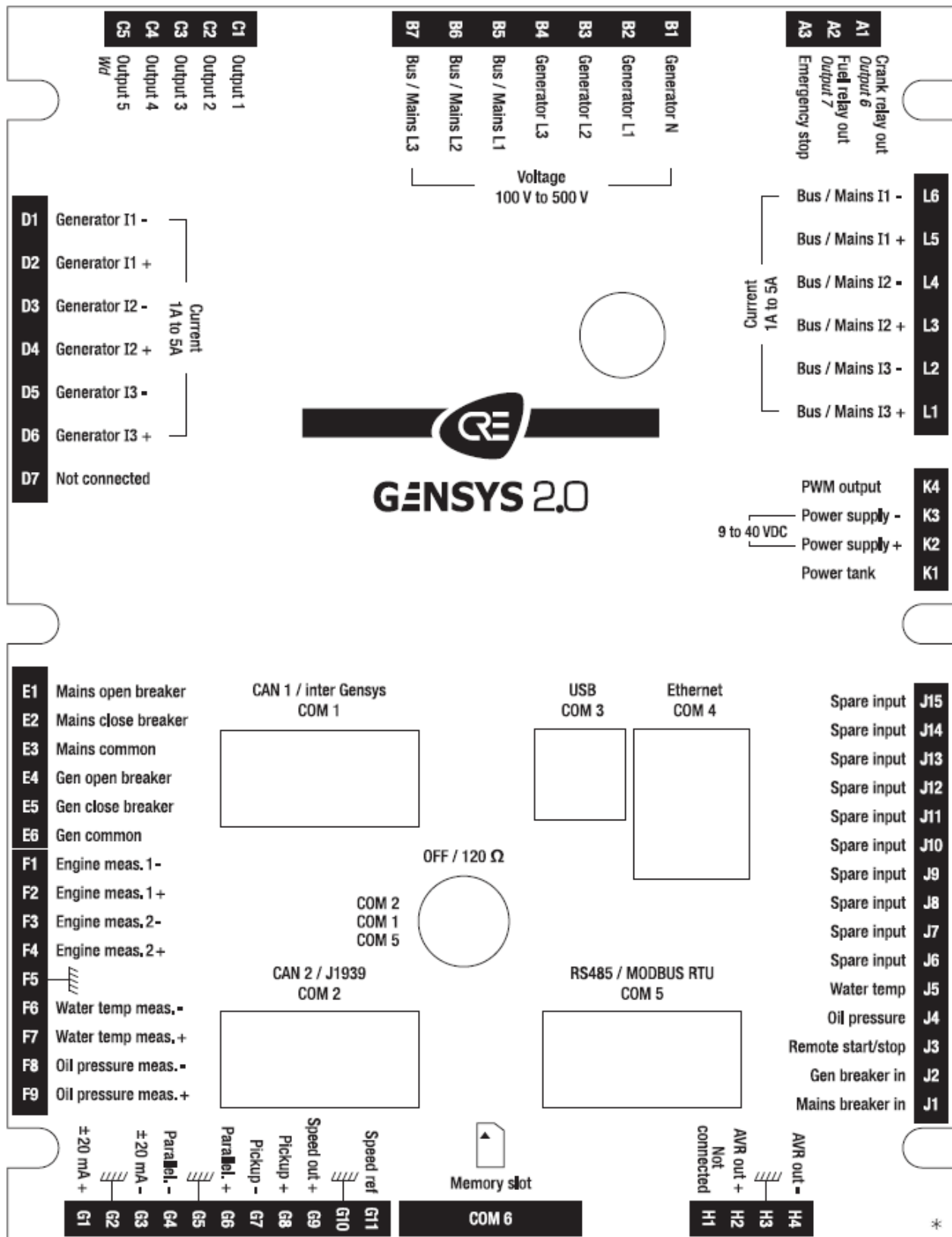
FIGURE 5 - FACE ARRIÈRE
