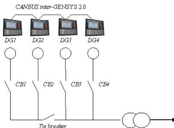
FIGURE 87 - CAN BUS INHIBITION SCHEMATIC (EXAMPLE)
